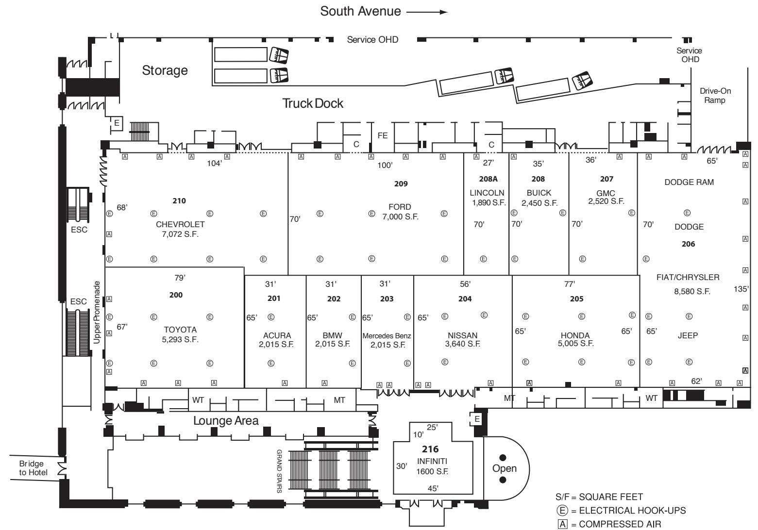
PRELIMINARY FLOORPLAN 2019 Spaces Marked
